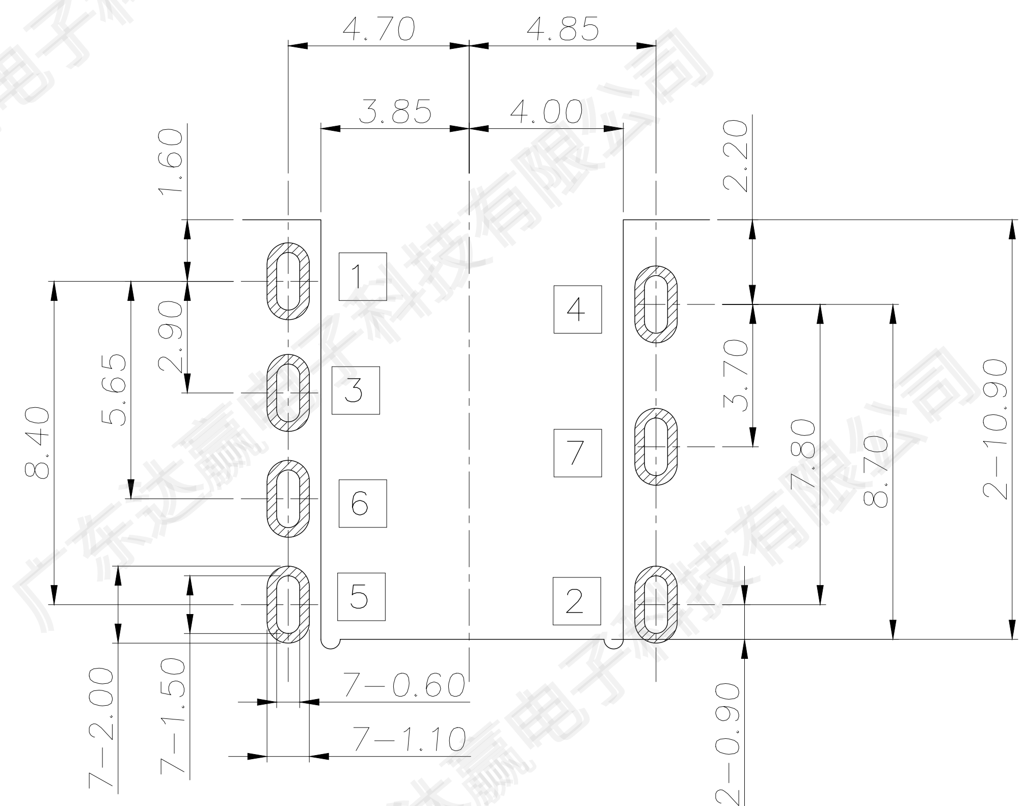
RECOMMENDED P.C.B LAYOUT (t=1.0mm) TOP VIEW (TOLRANCE: ±0.05)
