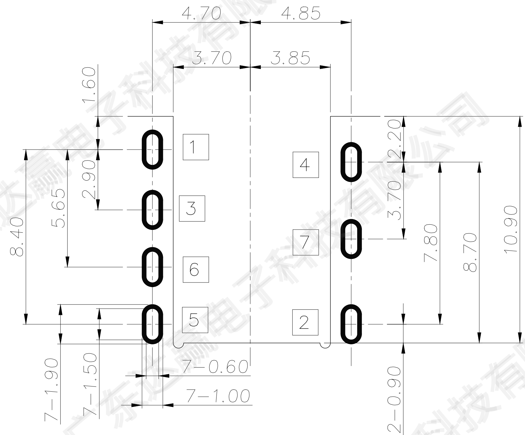
RECOMMENDED P. C. B LAYOUT TOP VIEW (TOLRANCE: ±0.05)
