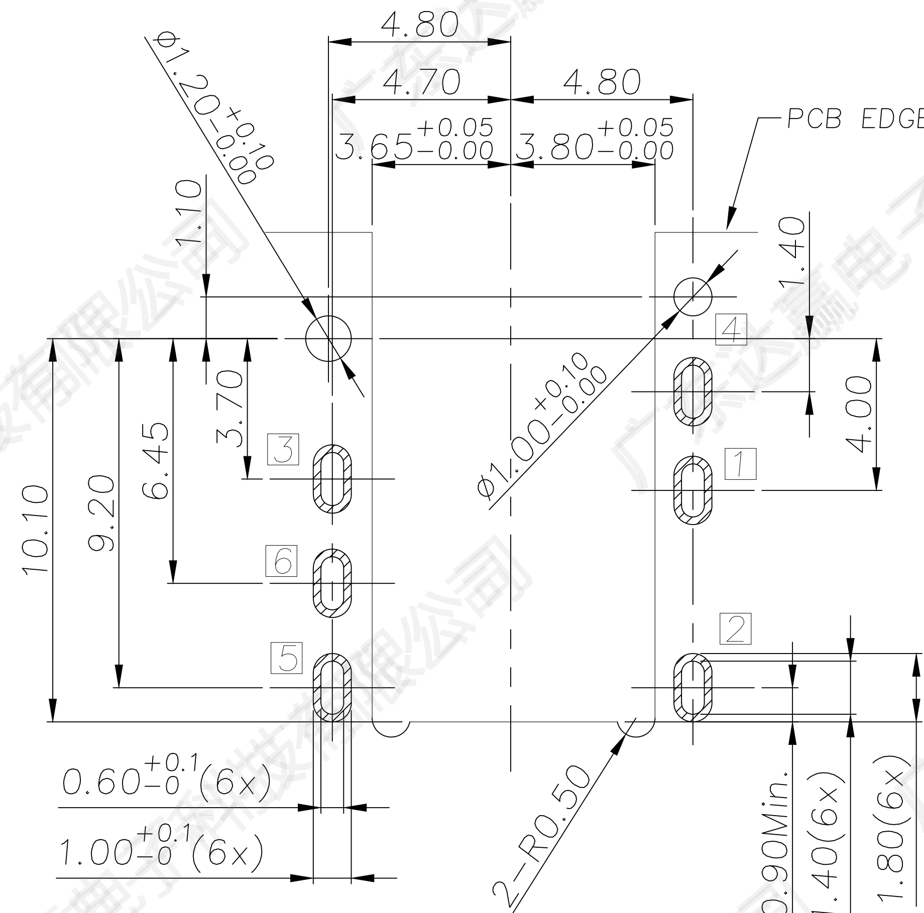
RECOMMENDED P.C.B. LAYOUT TOP VIEW (TOLRANCE: ±0.05)
